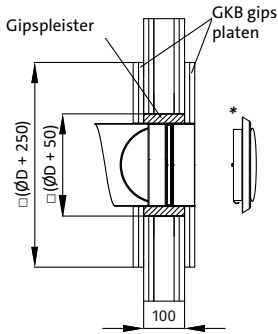
BFDC-V Montage in flexibele wand
