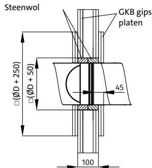
BFDC Montage in flexibele wand
