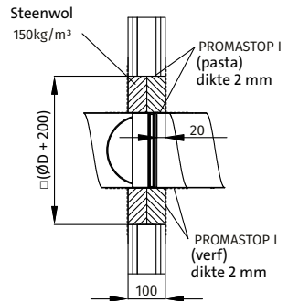
BFDC Montage in flexibele wand
