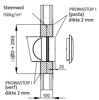
BFDC-V Montage in flexibele wand
