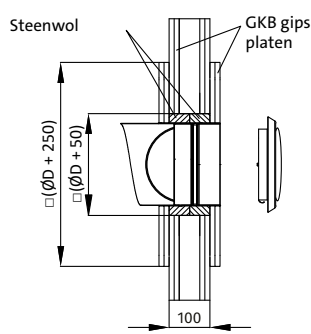
BFDC-V Montage in flexibele wand
